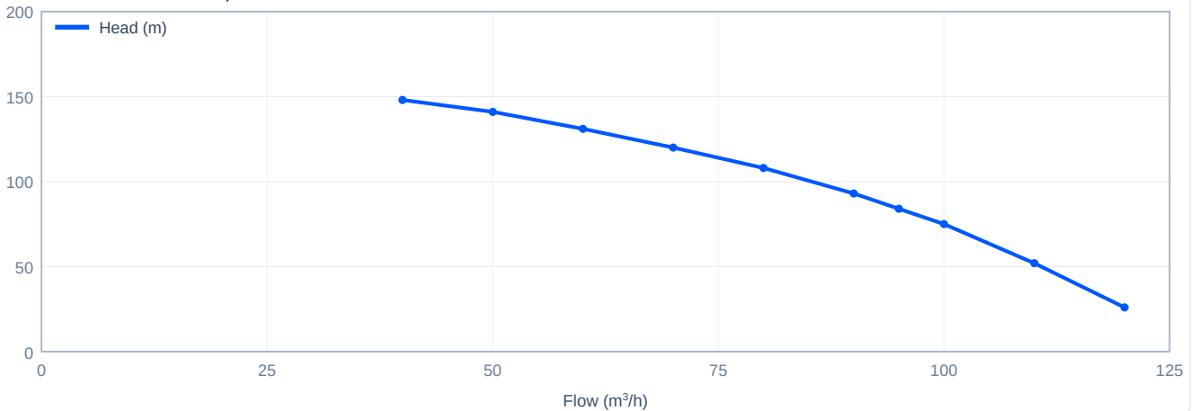
Head versus flow - SJ95-8, 50 Hz
