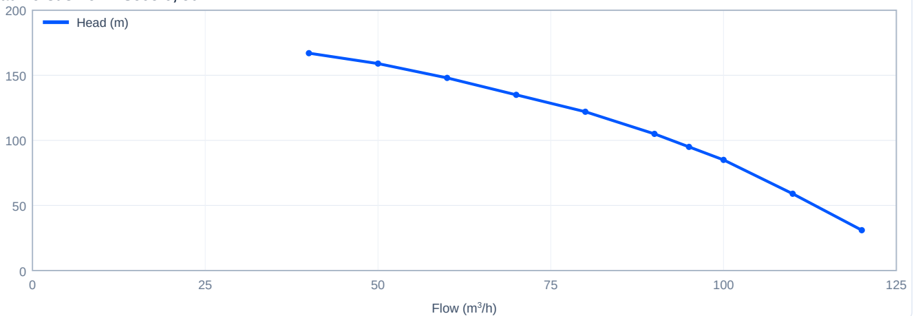
Head versus flow - SJ95-9, 50 Hz
