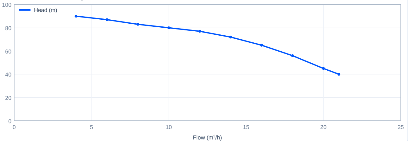
Head versus flow - SJ12-10, 60 Hz
