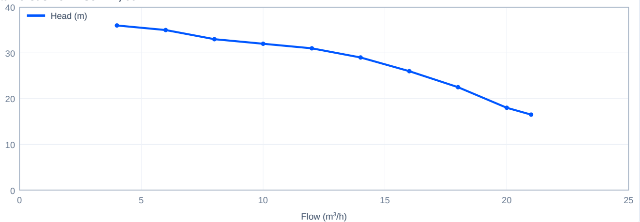
Head versus flow - SJ12-4, 60 Hz
