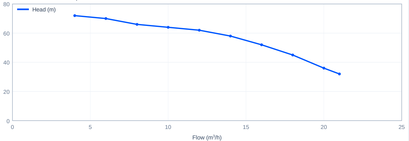
Head versus flow - SJ12-8, 60 Hz
