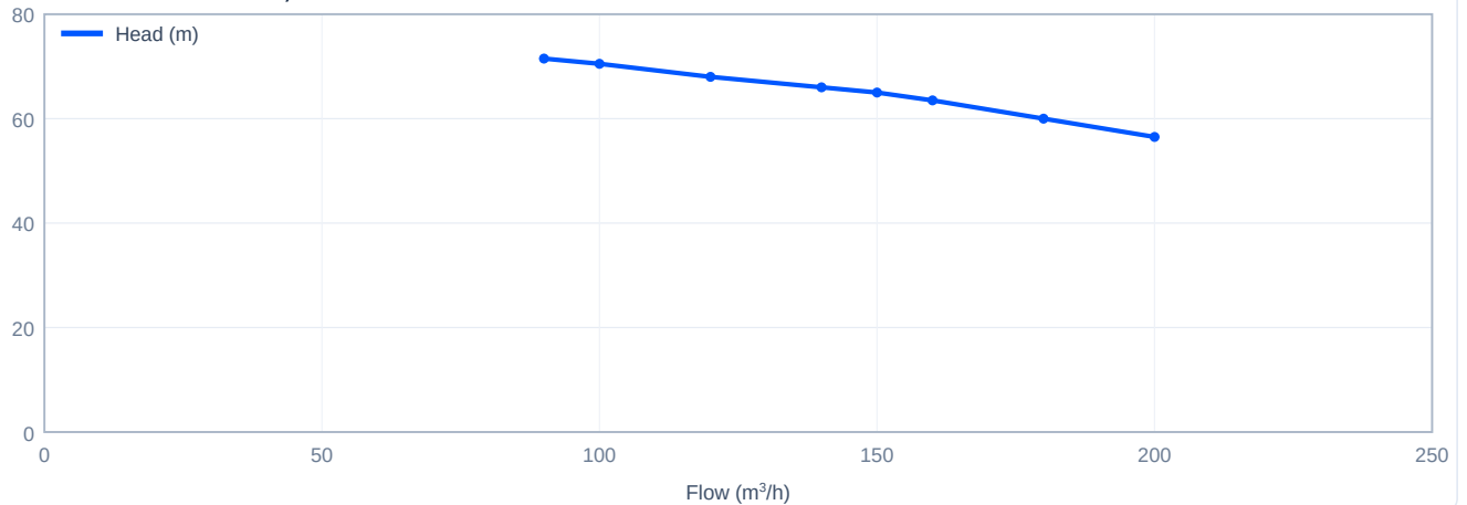
Head versus flow - SJ150-2, 60 Hz
