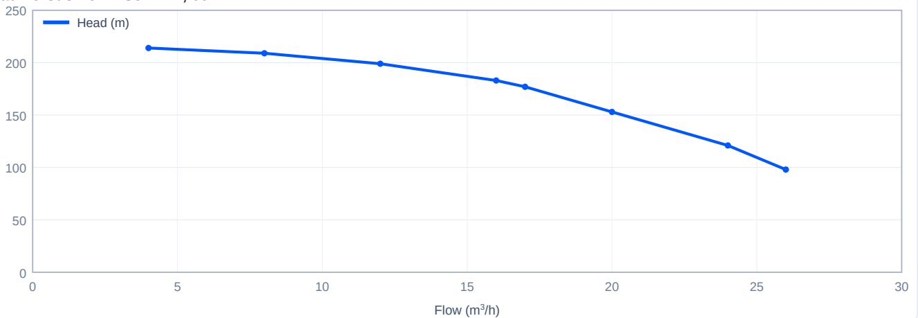
Head versus flow - SJ17-14, 60 Hz
