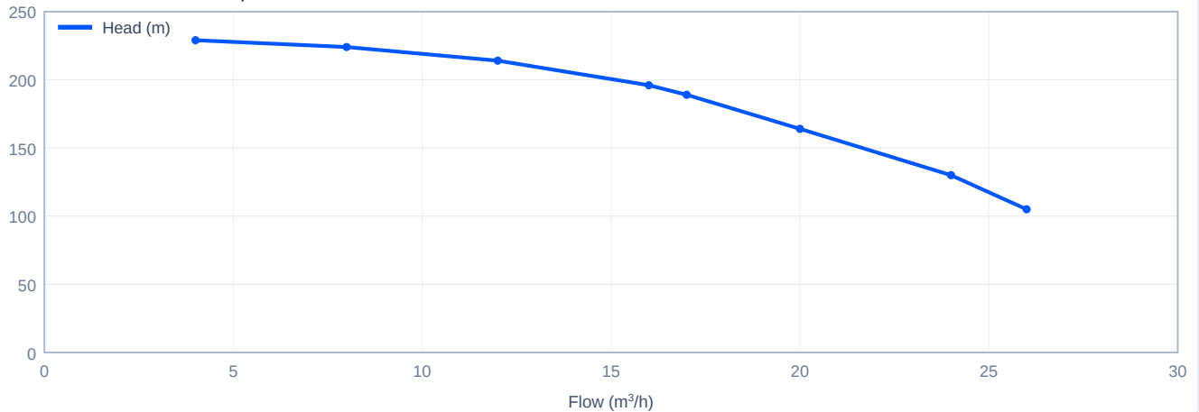
Head versus flow - SJ17-15, 60 Hz
