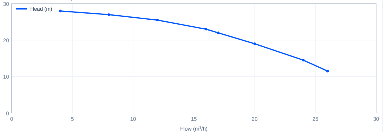
Head versus flow - SJ17-2, 60 Hz
