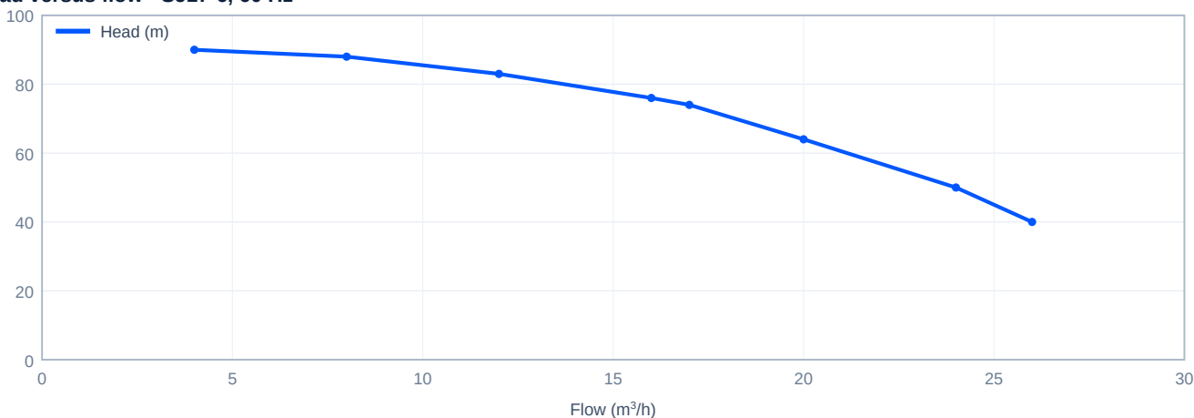
Head versus flow - SJ17-6, 60 Hz
