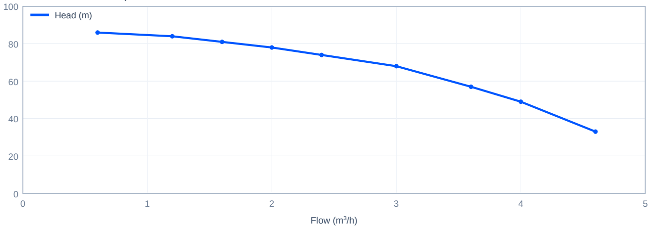
Head versus flow - SJ3-10, 60 Hz
