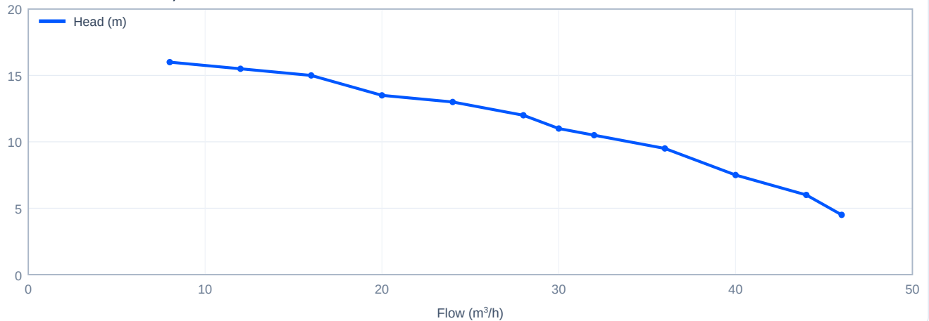
Head versus flow - SJ30-1, 60 Hz
