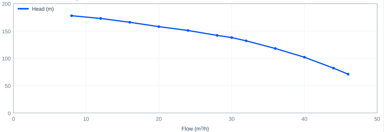
Head versus flow - SJ30-11, 60 Hz
