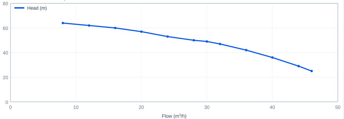
Head versus flow - SJ30-4, 60 Hz
