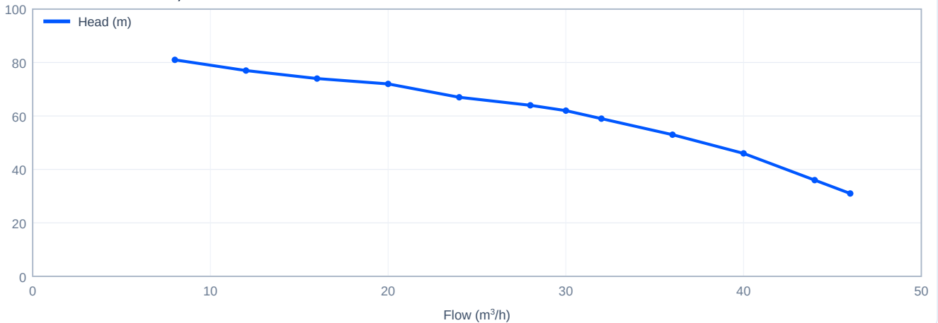
Head versus flow - SJ30-5, 60 Hz
