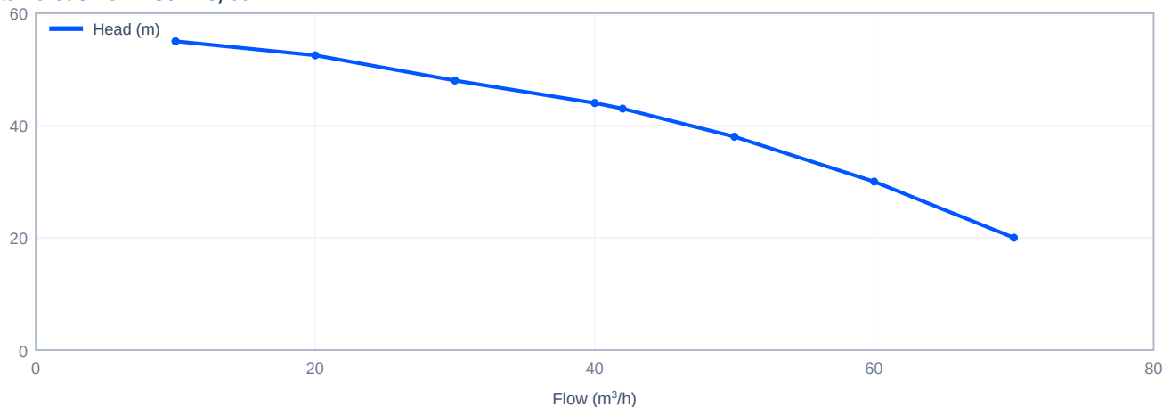
Head versus flow - SJ42-3, 60 Hz
