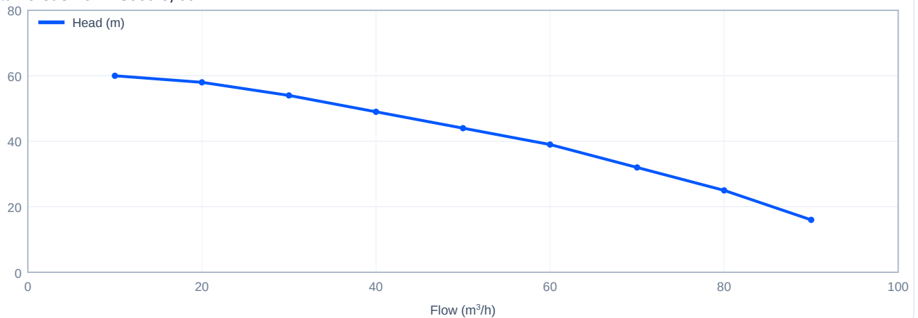
Head versus flow - SJ60-3, 60 Hz
