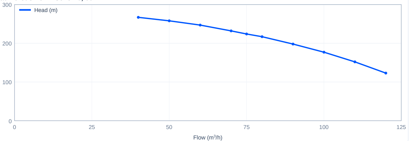
Head versus flow - SJ75-10, 60 Hz
