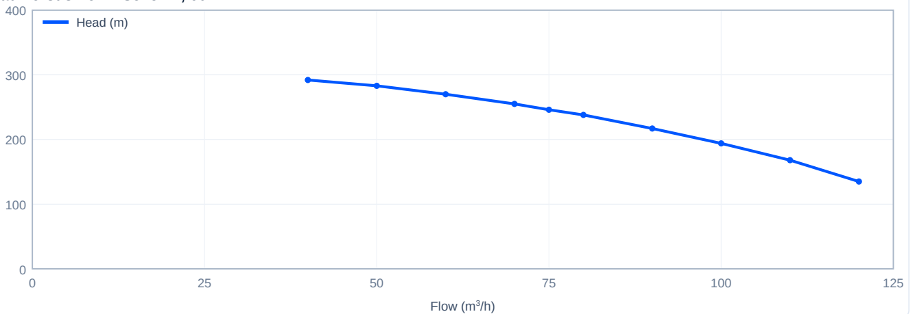
Head versus flow - SJ75-11, 60 Hz
