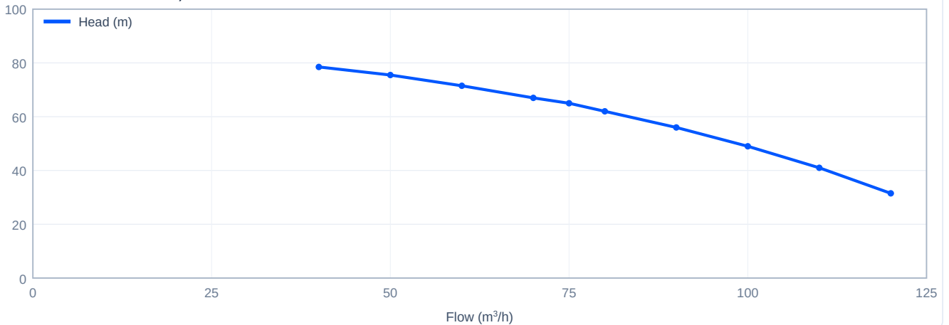
Head versus flow - SJ75-3, 60 Hz
