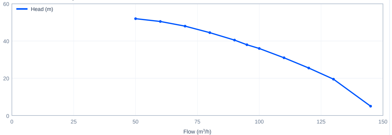
Head versus flow - SJ95-2, 60 Hz
