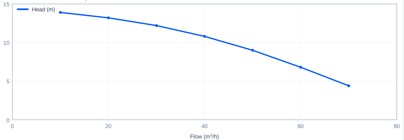
Head versus flow - TD100-9/2, 50 Hz
