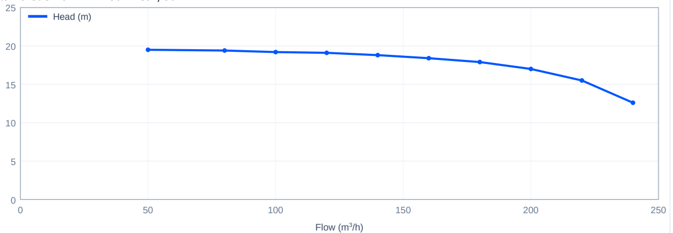
Head versus flow - TD150-17G/4, 50 Hz
