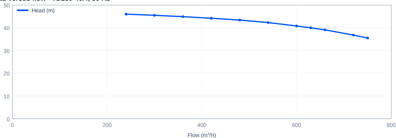
Head versus flow - TD250-40/4, 50 Hz
