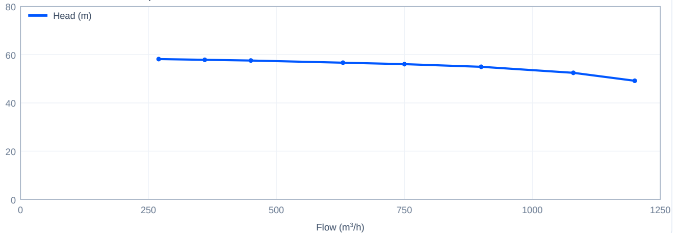
Head versus flow - TD300-55/4, 50 Hz
