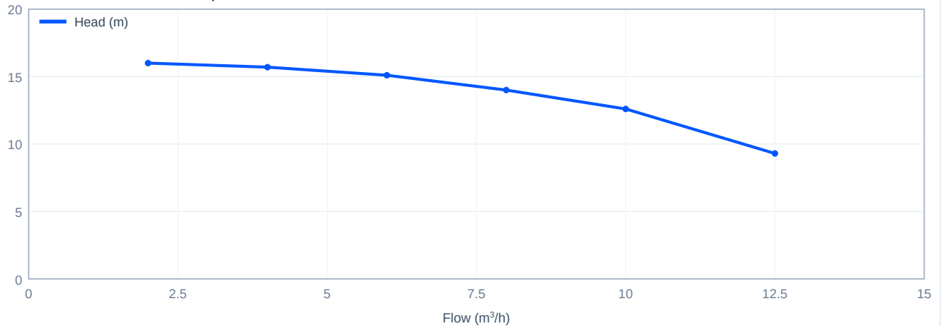
Head versus flow - TD32-14G/2, 50 Hz
