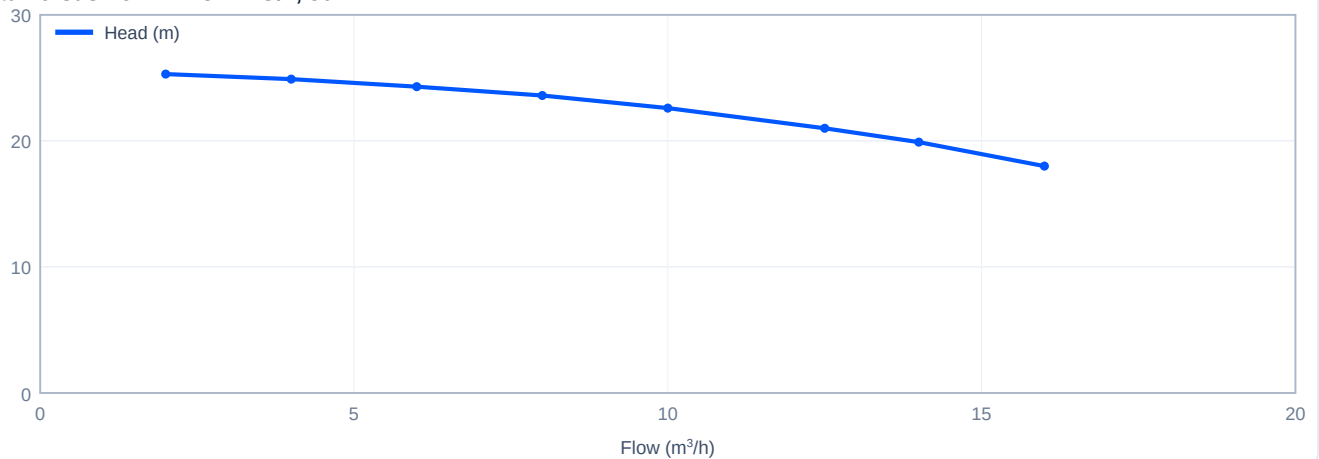
Head versus flow - TD32-21G/2, 50 Hz
