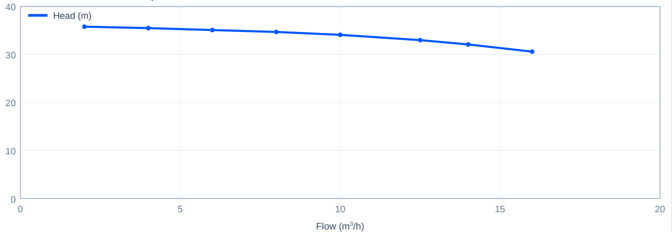
Head versus flow - TD32-33G/2, 50 Hz
