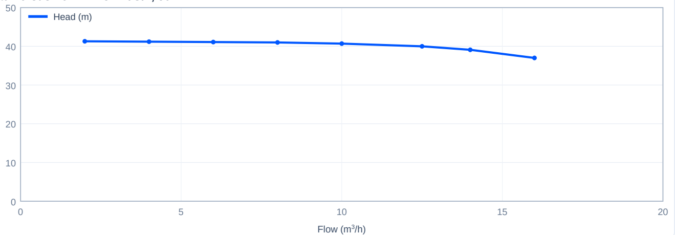
Head versus flow - TD32-40G/2, 50 Hz
