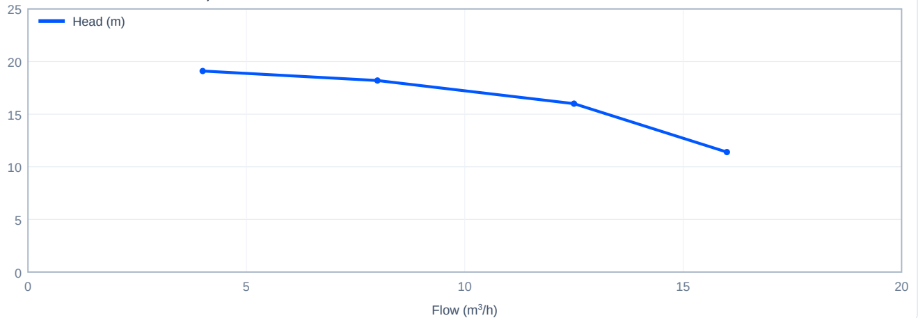
Head versus flow - TD40-16G/2, 50 Hz
