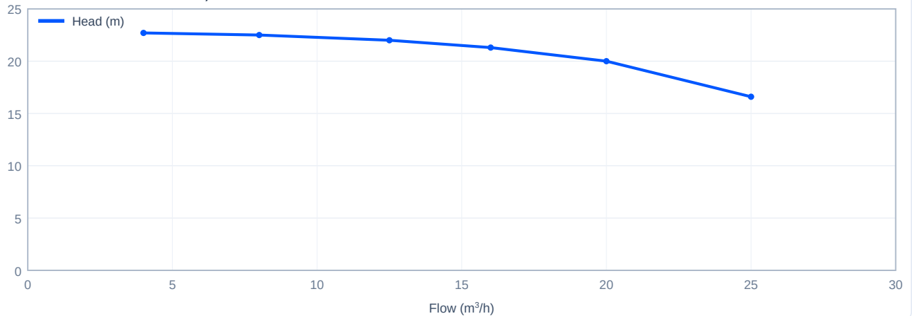
Head versus flow - TD40-20G/2, 50 Hz
