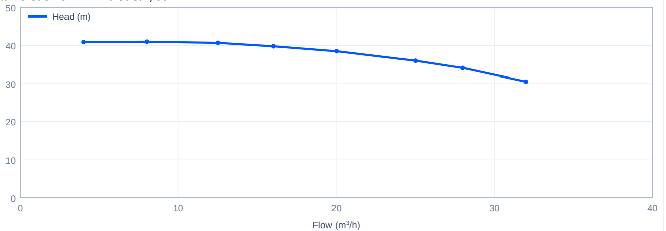
Head versus flow - TD40-36G/2, 50 Hz
