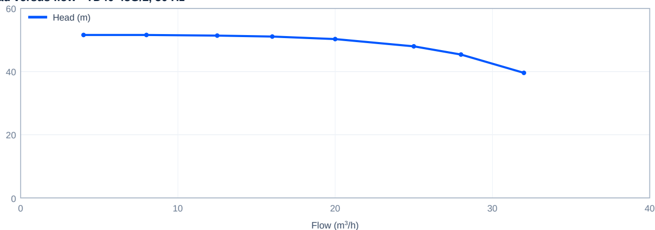
Head versus flow - TD40-48G/2, 50 Hz
