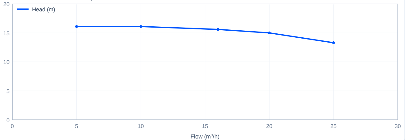
Head versus flow - TD50-15G/2, 50 Hz
