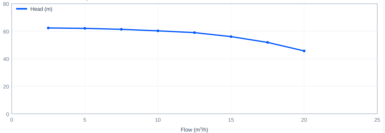
Head versus flow - TD50-59G/2, 50 Hz
