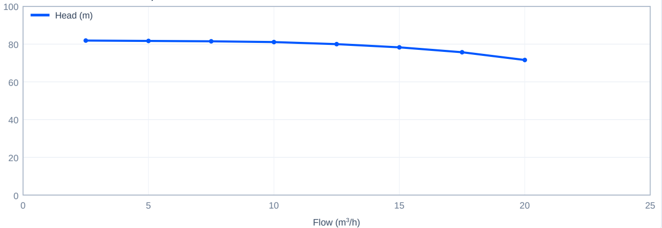
Head versus flow - TD50-80G/2, 50 Hz
