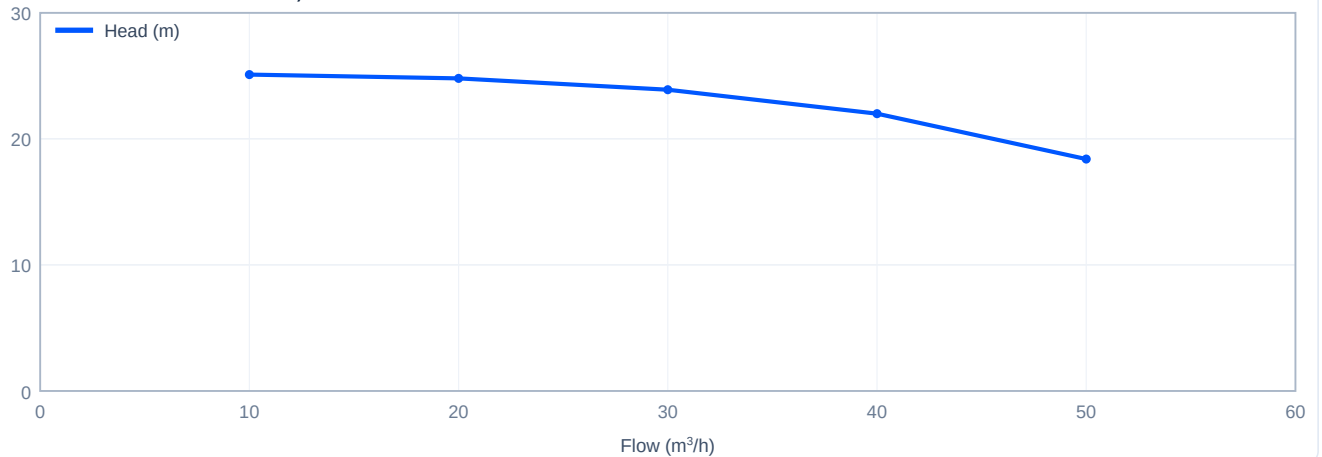
Head versus flow - TD65-22G/2, 50 Hz
