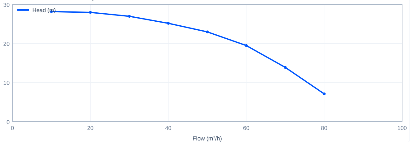
Head versus flow - TD80-23G/2, 50 Hz
