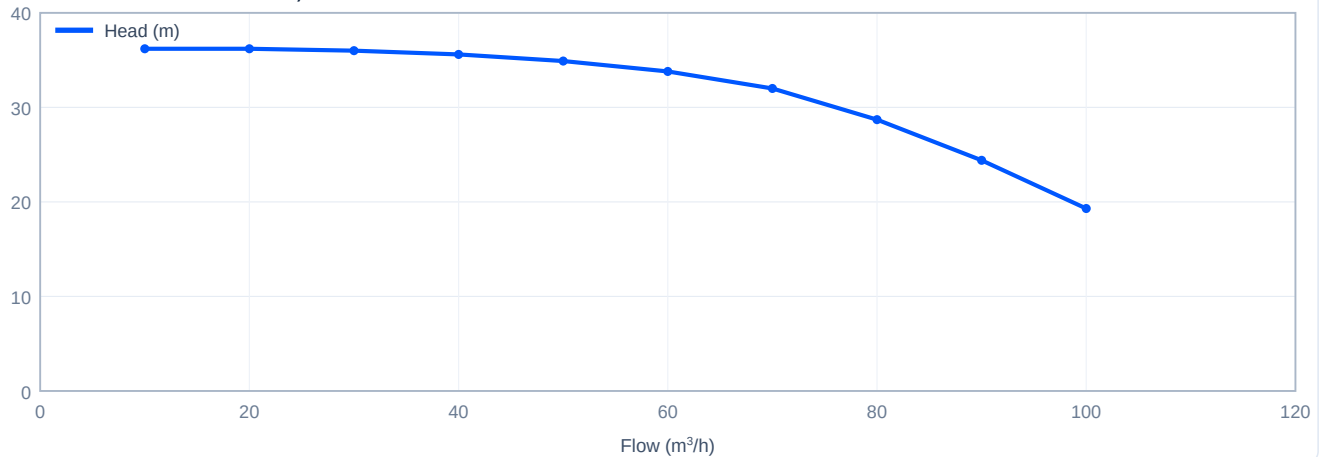
Head versus flow - TD80-32G/2, 50 Hz
