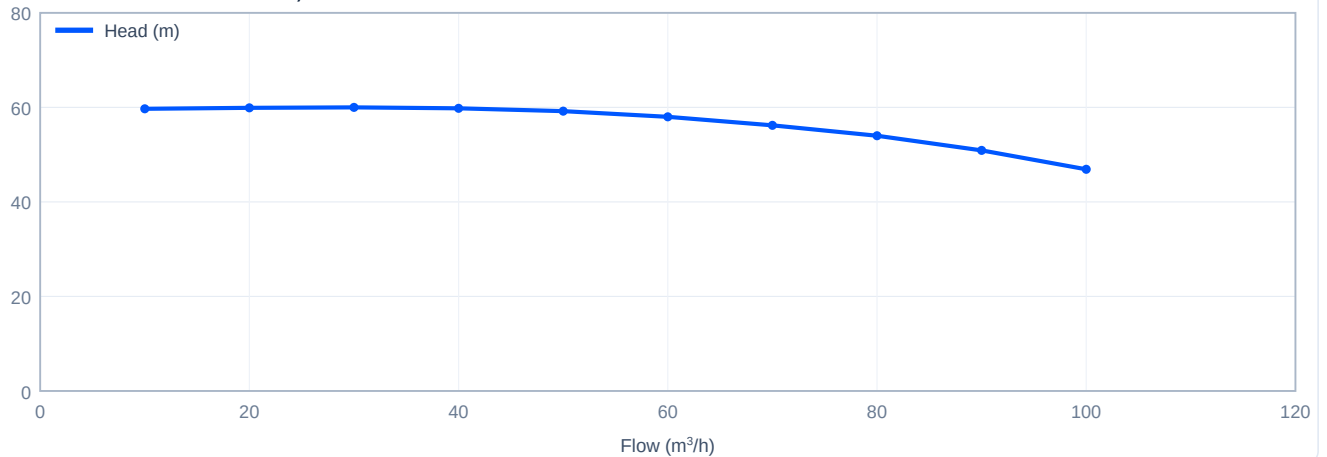
Head versus flow - TD80-54G/2, 50 Hz
