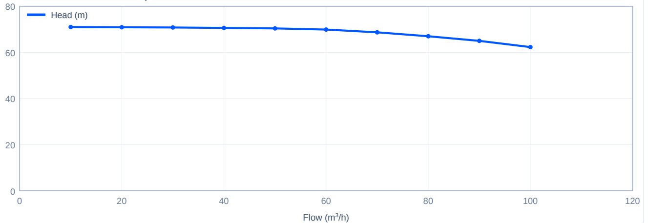
Head versus flow - TD80-67G/2, 50 Hz
