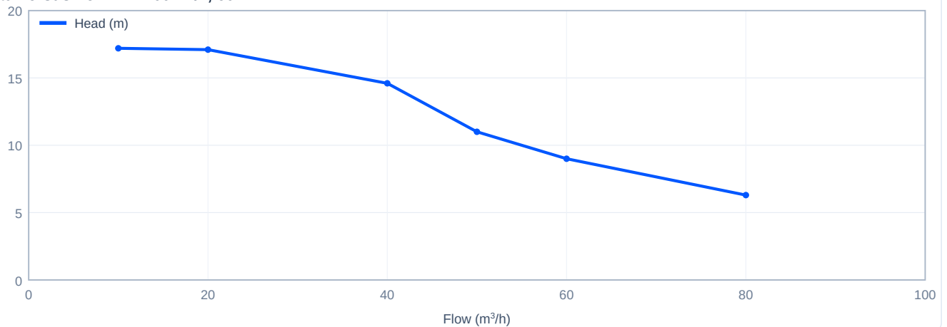
Head versus flow - TD100-11/2, 60 Hz
