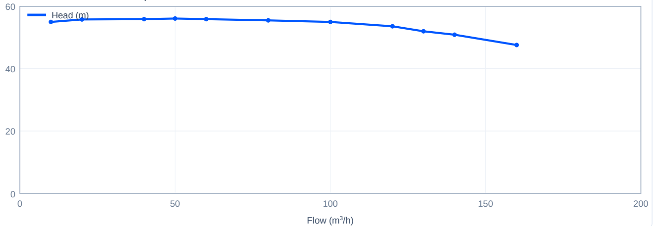
Head versus flow - TD100-52/2, 60 Hz
