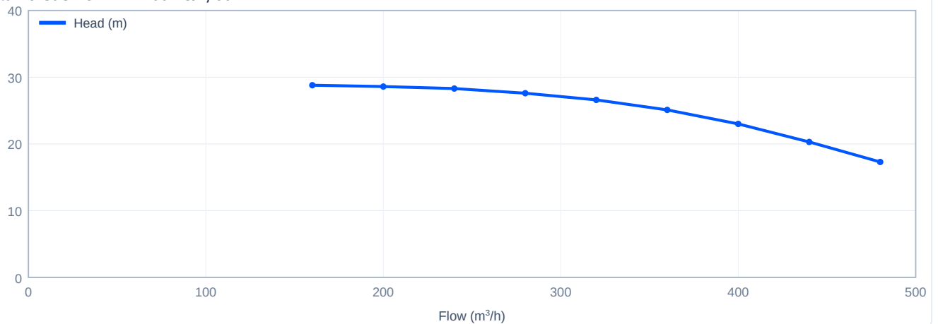
Head versus flow - TD200-23/4, 60 Hz
