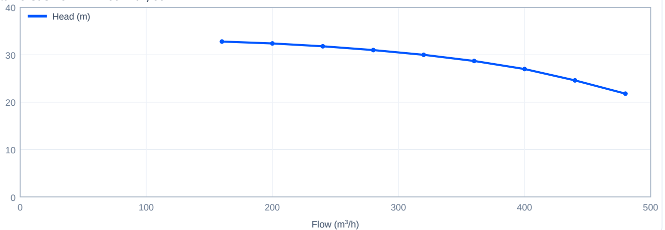
Head versus flow - TD200-27/4, 60 Hz
