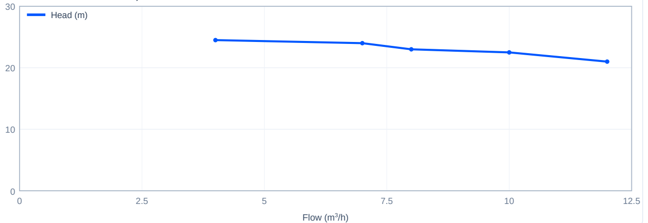
Head versus flow - TD32-24/2, 60 Hz
