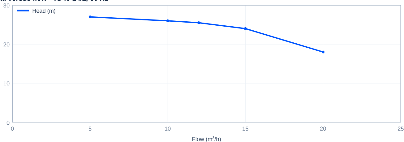
Head versus flow - TD40-24/2, 60 Hz
