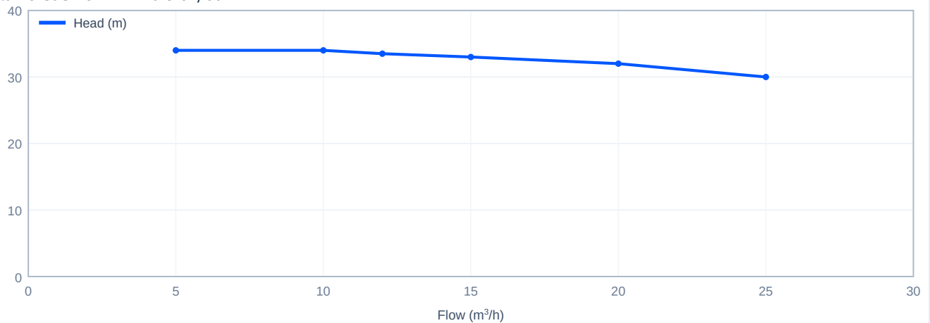
Head versus flow - TD40-32/2, 60 Hz
