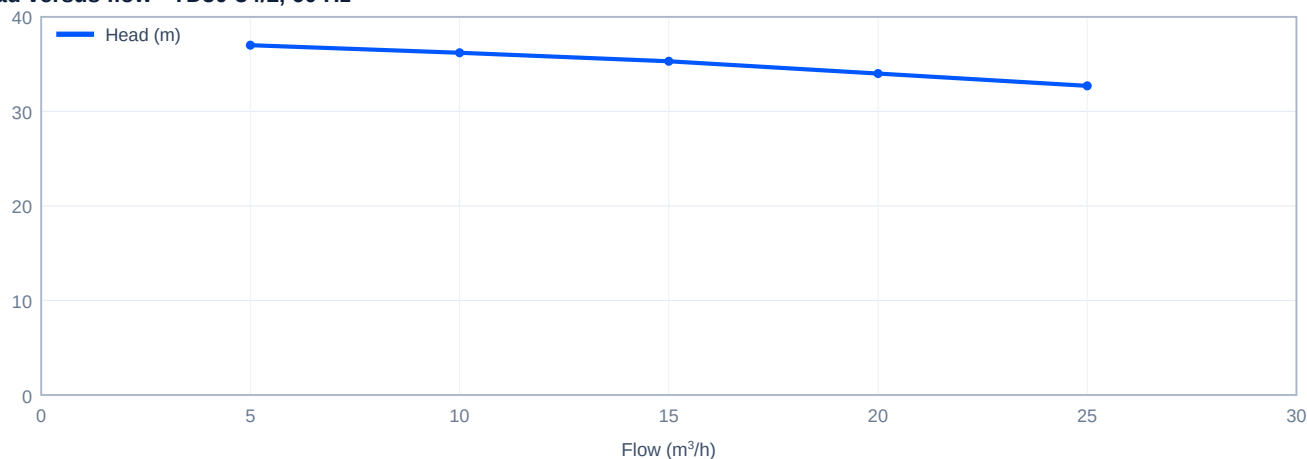
Head versus flow - TD50-34/2, 60 Hz
