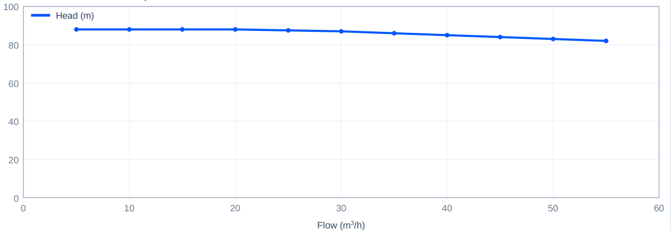
Head versus flow - TD50-84/2, 60 Hz
